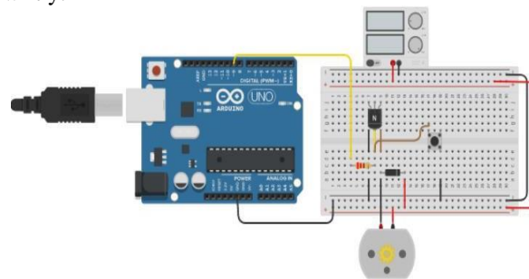
Fig.9. Emergency Switch
