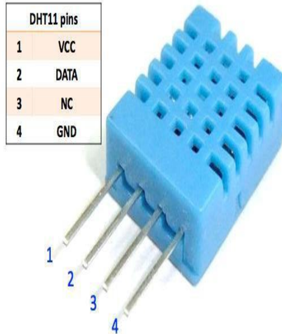
Fig.4. DHT-11 Sensor.
