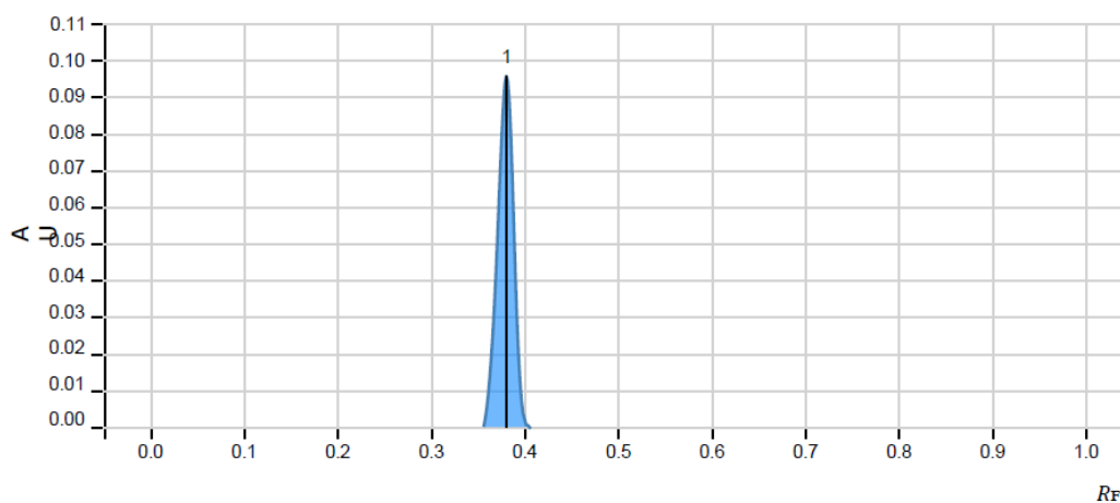
Figure 3: HPLC Chromatograms of Azadirachtin(standard) at Volume 4.0 µL
